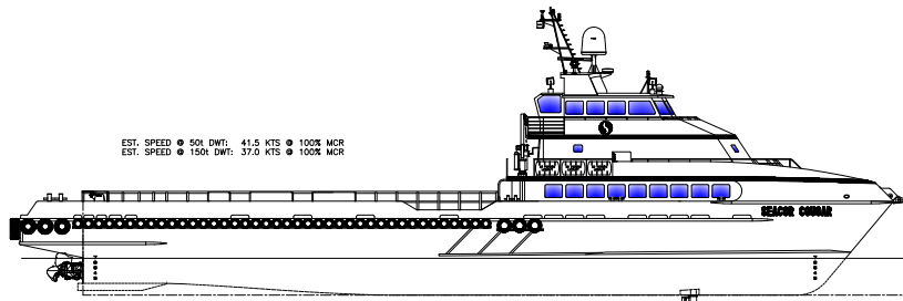
OUTBOARD PROFILE
