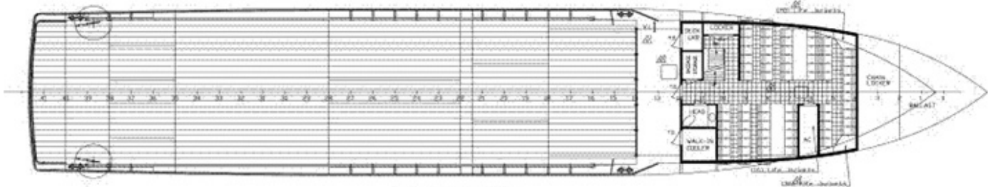
MAIN DECK PLAN
