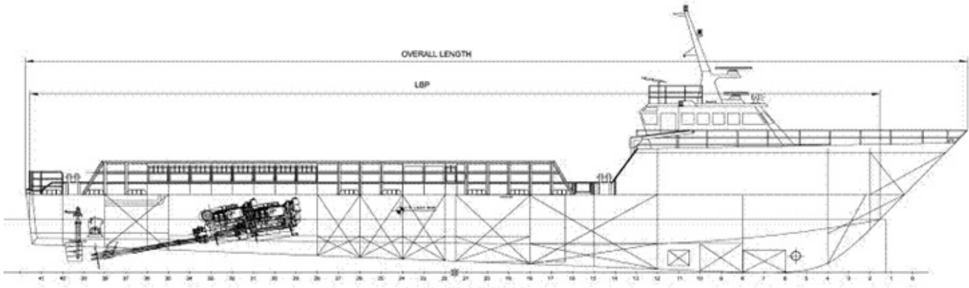
OUTBOARD PROFILE
