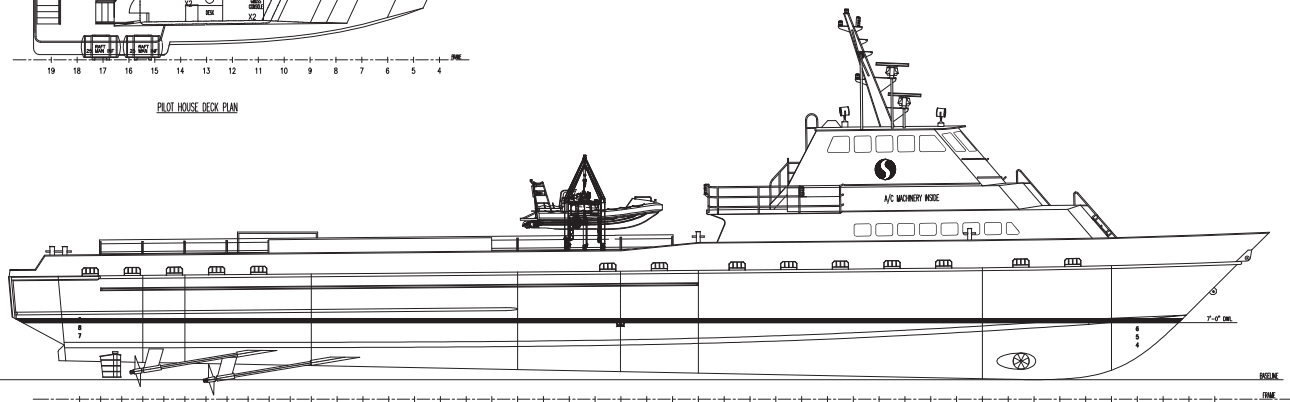
OUTBOARD PROFILE
