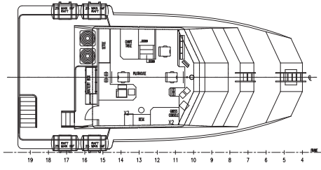
PILOT HOUSE DECK PLAN
